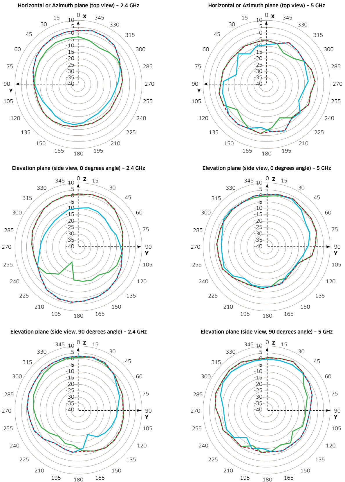
Figure 1. OmniAccess AP1201L antenna pattern plots
